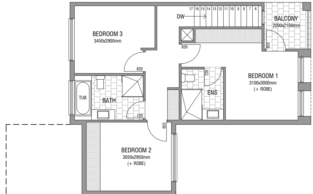
UPPER FLOOR PLAN DWELLING 2&4
