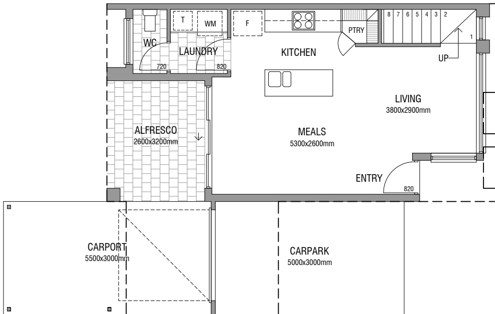
GROUND FLOOR PLAN DWELLING 2&4
