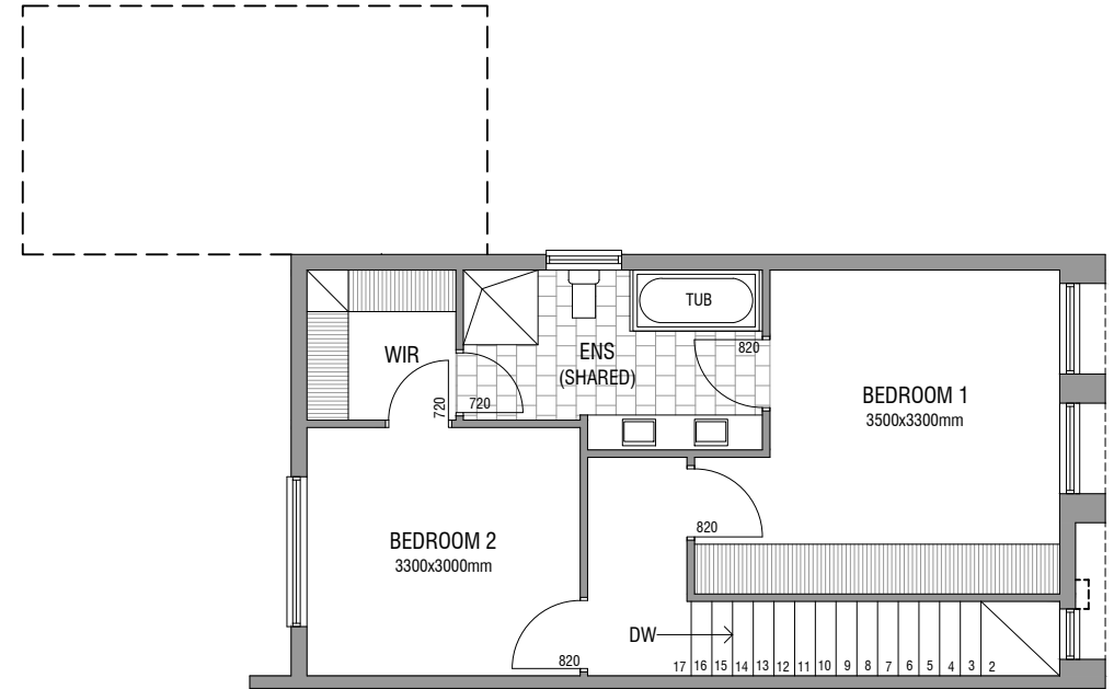
UPPER FLOOR PLAN DWELLING 3&5
