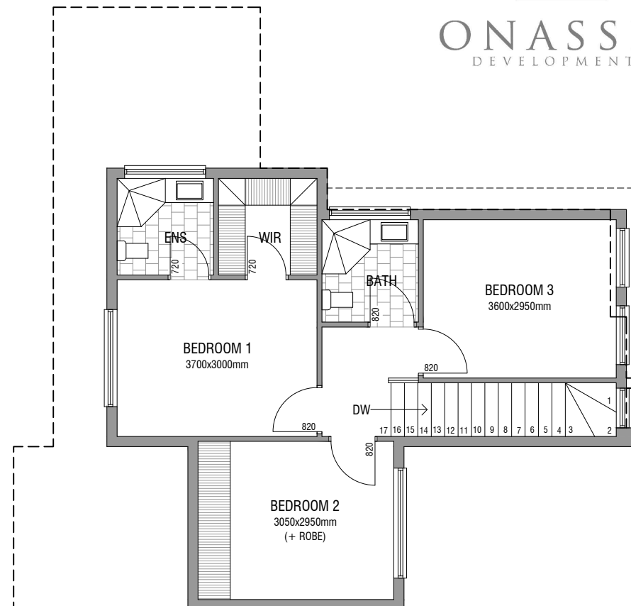
UPPER FLOOR PLAN DWELLING 6
