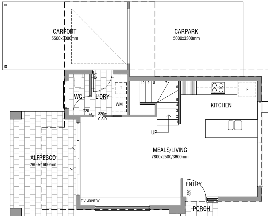
GROUND FLOOR PLAN DWELLING 1
